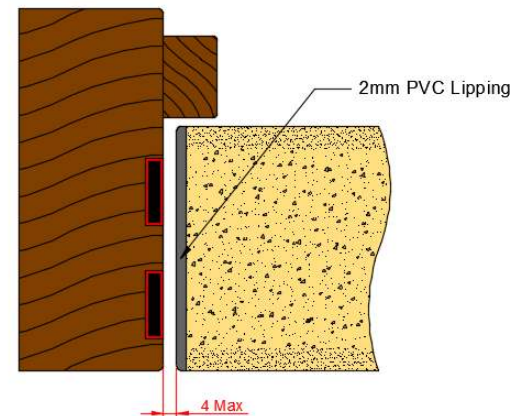
PVC Lipping Option 2
